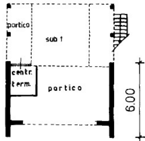
860 piano terra H= 210
