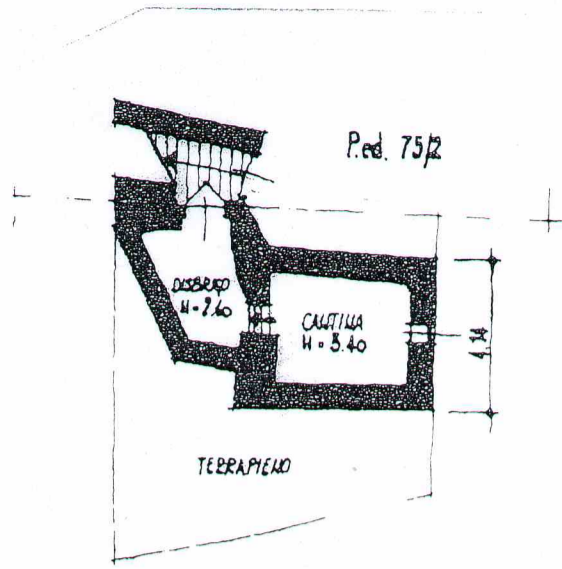
PIANO INTERRATO H = Varia
