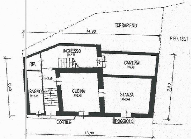
PIANO TERRA H=VARIA
